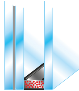
SS 44.2/16/10 PTR+(coef Ug=1,1) (Rw 41db)
