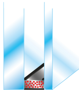
10/16/4 PTR+(coef Ug=1,1) (Rw 35db)
